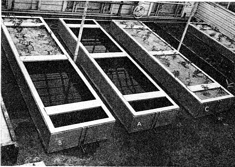
Fig. 7. General arrangement of tank equipment and method of planting: A, a frame supporting a wire screen fits over the metal tank (fig. 6, A) filled with the nutrient solution; B, tomato plants are placed with their roots immersed in the nutrient solution; a layer of excelsior is spread over the netting, as shown in the far end of the tank; C, the planting is completed by spreading a layer of rice hulls over the excelsior.
